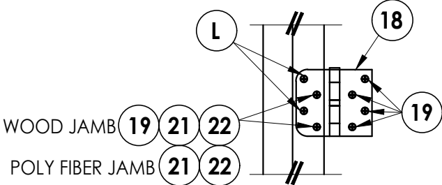
HINGE DETAIL
