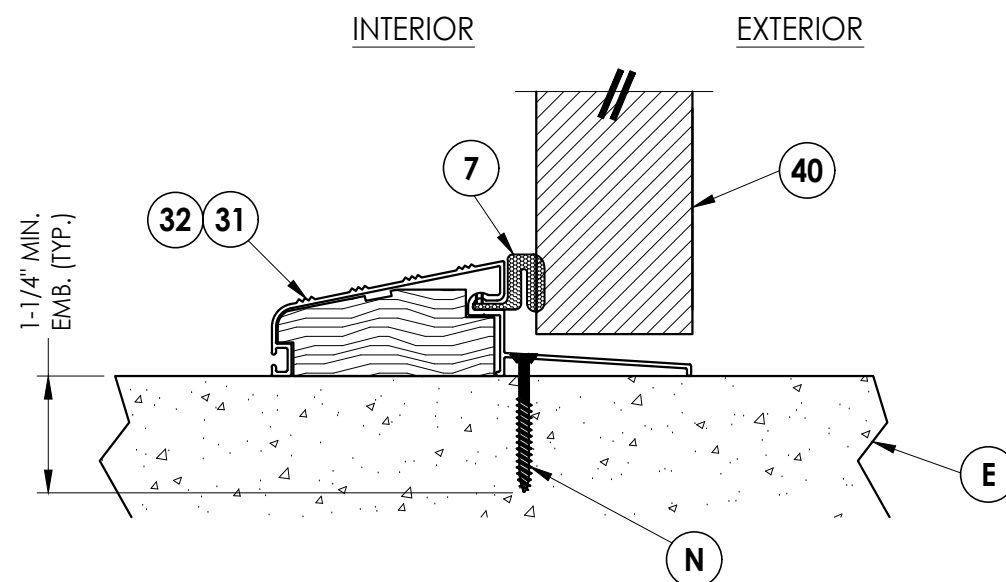
4 VERTICAL CROSS SECTION 6 Outswing configuration
