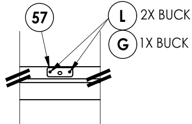
DETAIL 1 Astragal Strike Plate
