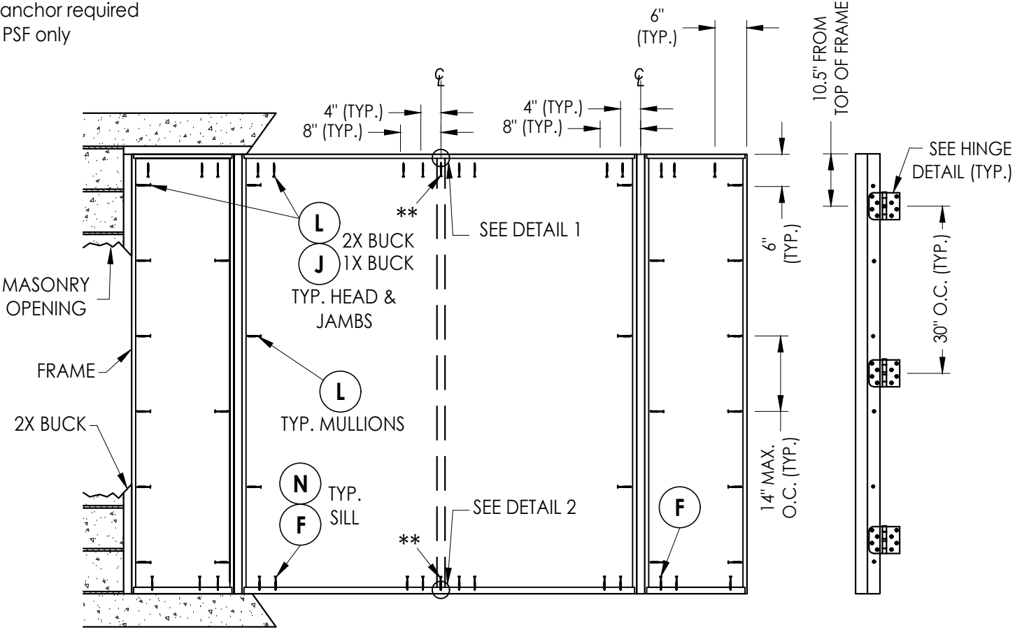
FRAME ANCHORING Masonry construction
