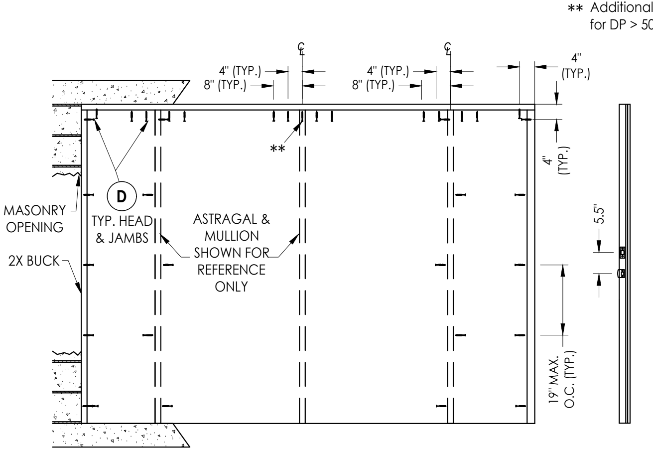
BUCK ANCHORING
