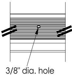
DETAIL 2 Astragal Bolt Hole Outswing
