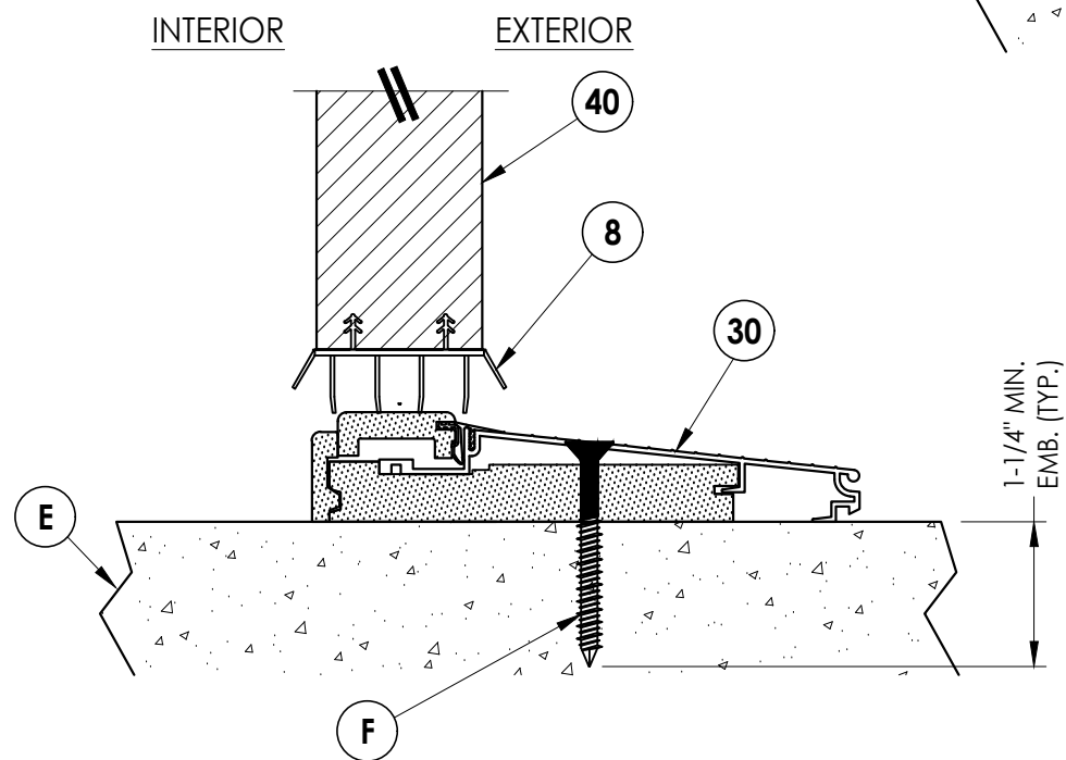
3 VERTICAL CROSS SECTION 6 Inswing configuration
